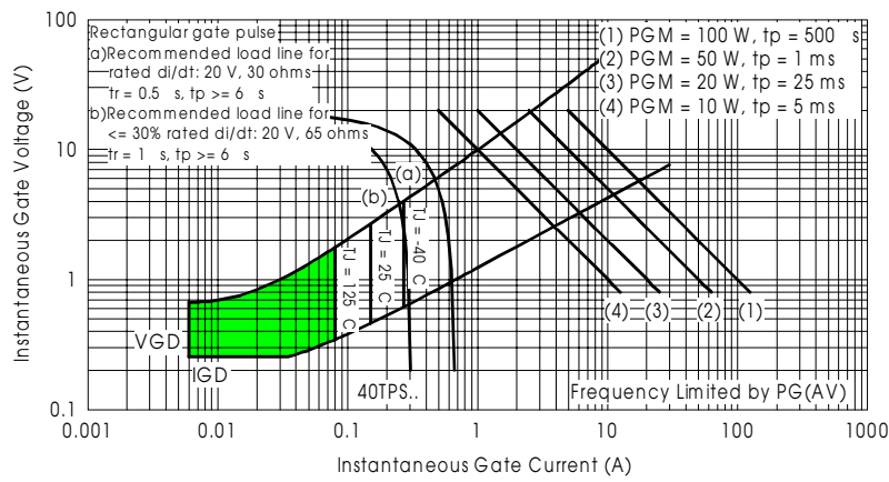
Fig. 8 - Gate Characteristics
